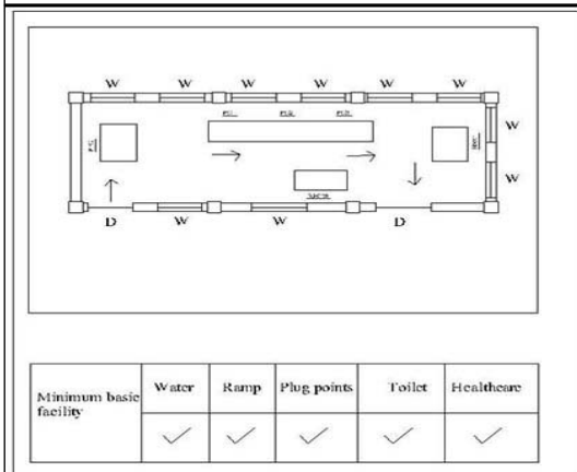
CAD View
