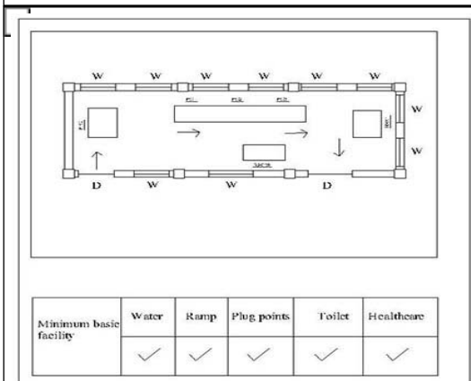
CAD View
